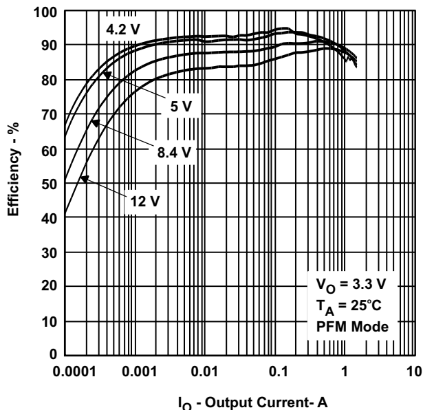
TPS62111 Efficiency vs Output Current
