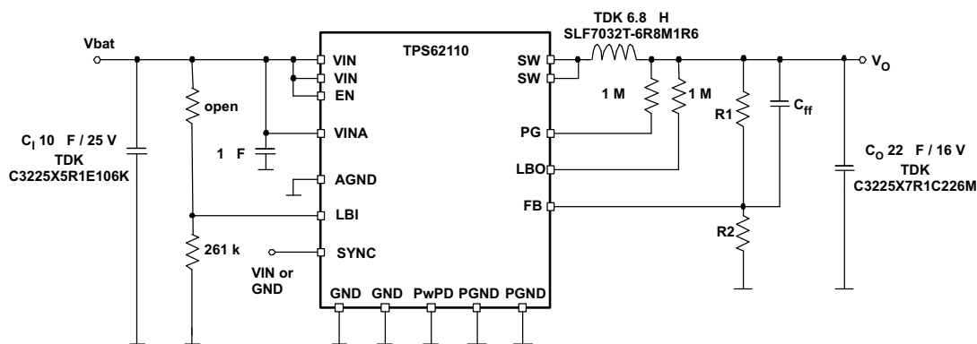
Figure 17. Test Setup
